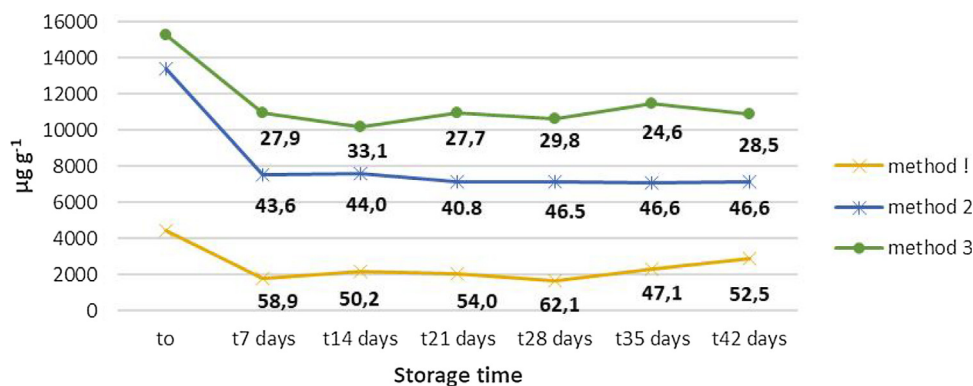
Fig. 5. Bedrocan's THC trends during storage at 4 °C in different cannabis oil preparation methods.
